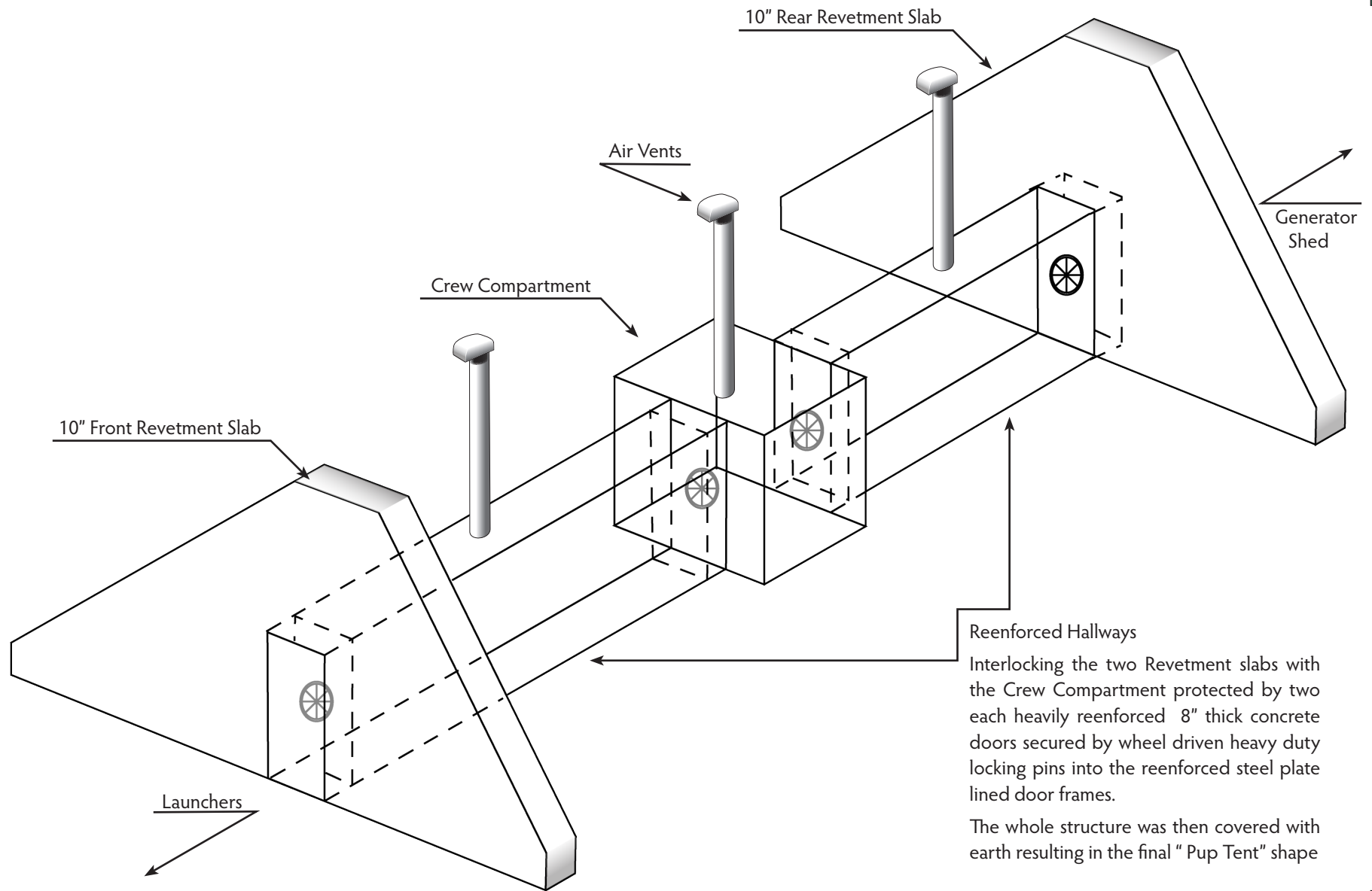
Launching Area Section Revetment Plan
