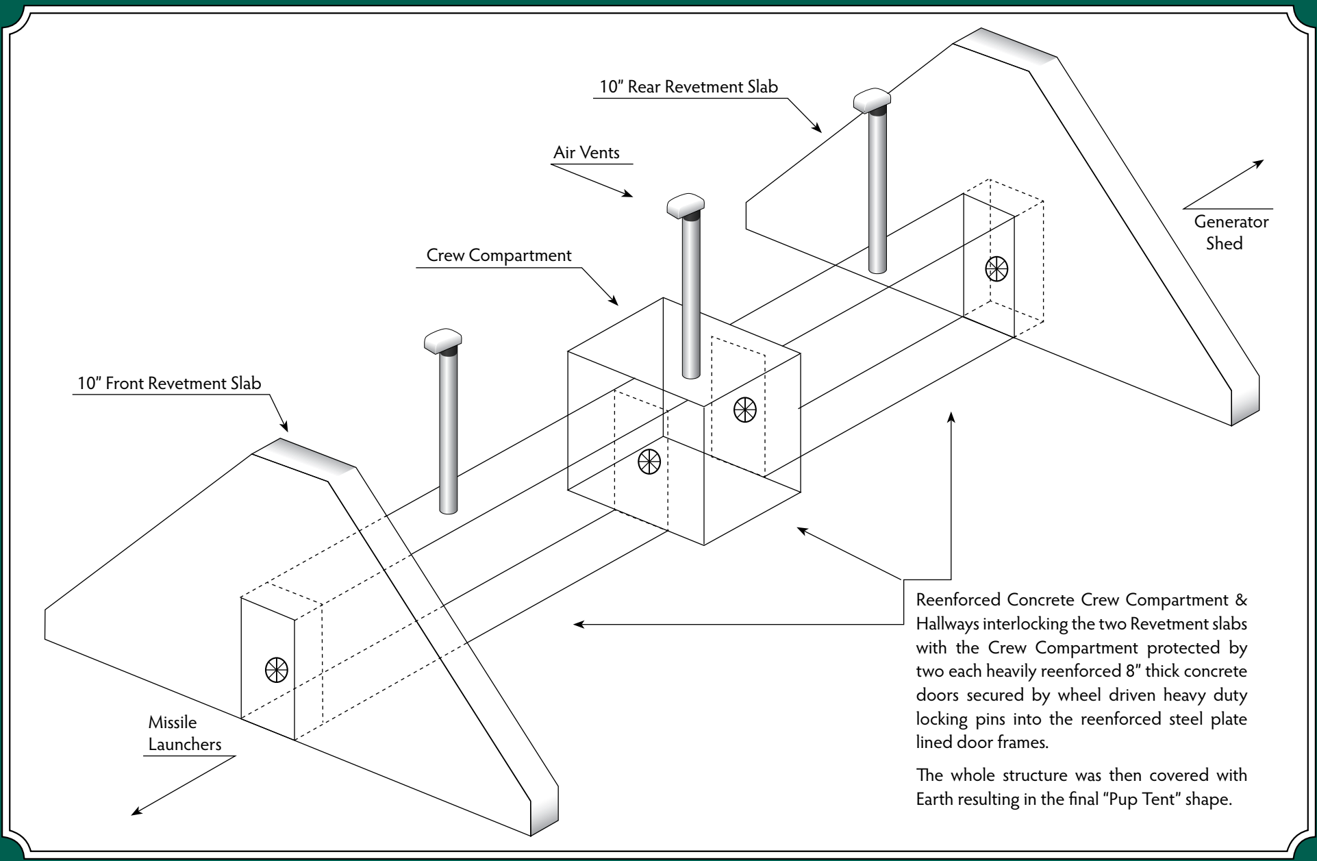
Launching Area Section Revetment Plan
